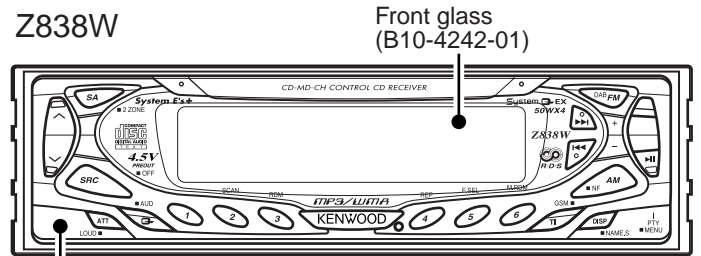
Panel Assy (A64-2689-11)
